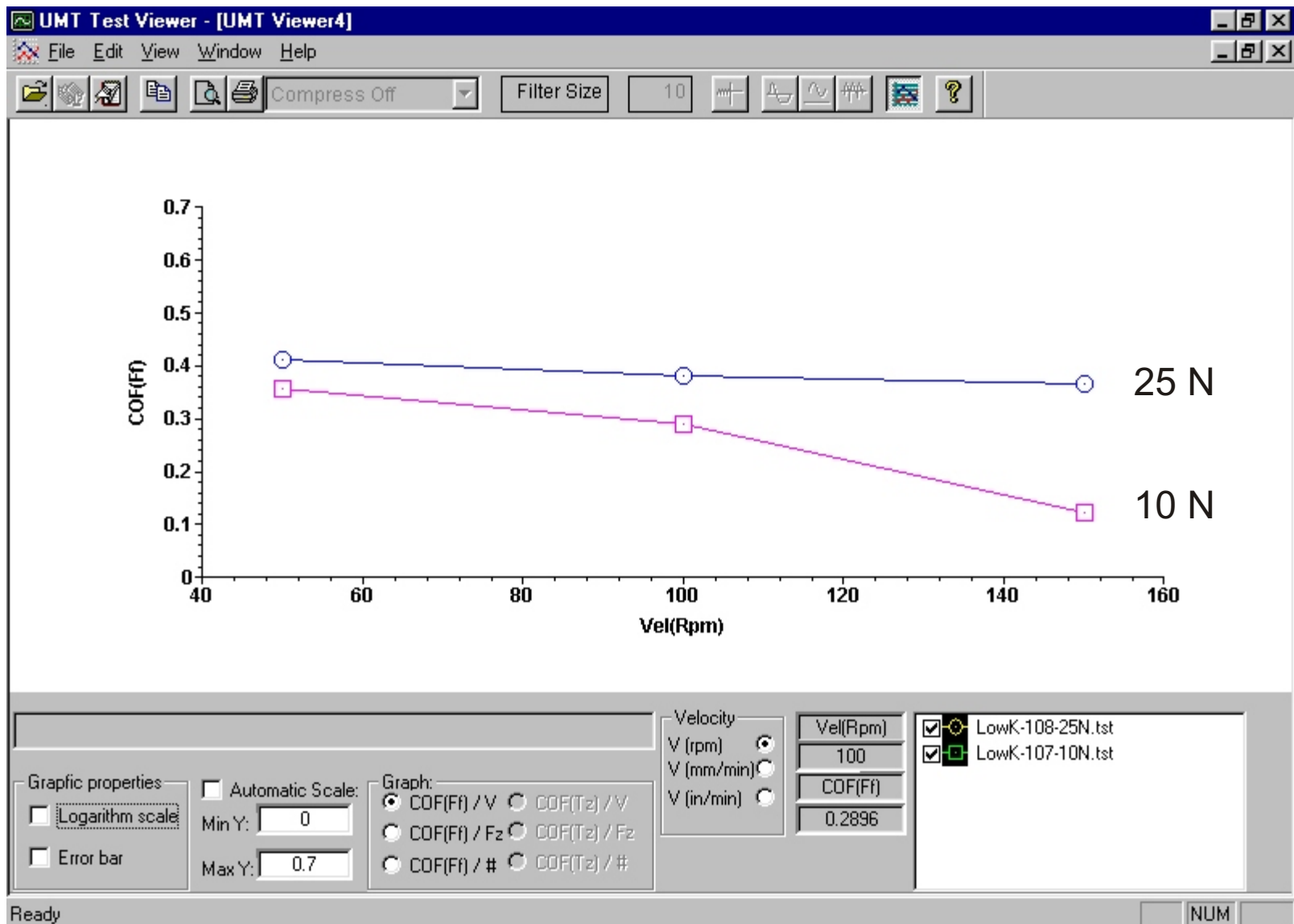
Fig. 1 Plots of Friction Coefficient
